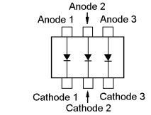
HN2D01FU (A1) (D1040)
