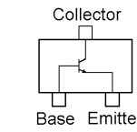
2SC4617 (BR) (Q1040, 1041, 1042) 2SC4915 (QY) (Q1017, 1020, 1021, 1022, 1023, 1028, 1035)
